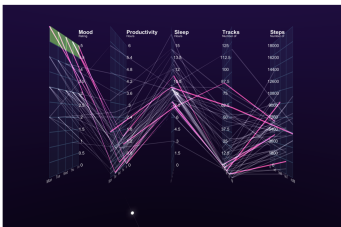
Figure 5: The user has brushed a region at the top of the Mood y-axis, across all days of the week (z-axis). As a result, highlighted lines emphasize values in other dimensions for all days when Mood was high.
